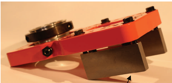
Tack-bars installed
